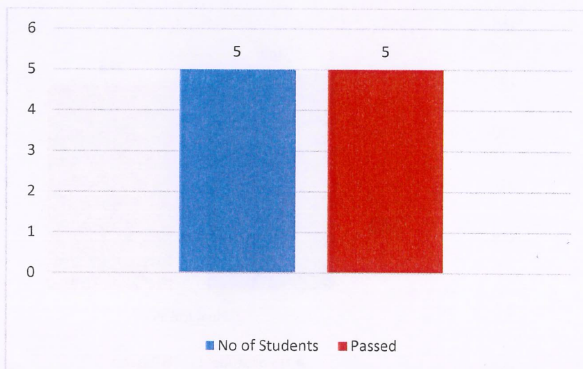
Graph 3 : DM/MCh Result
