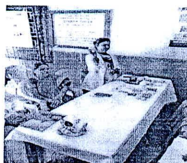
Quiz
